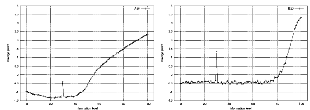
Figure 6. Left Graph. Income distribution among a human subject (Player 30) and middle-value strategy agents. Right Graph. Income distribution among a human subject (Player 30) and either-end strategy agents
